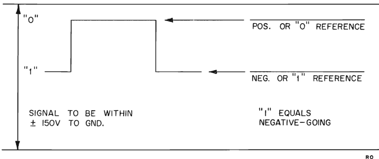
Figure 3-1. Reference Levels.
